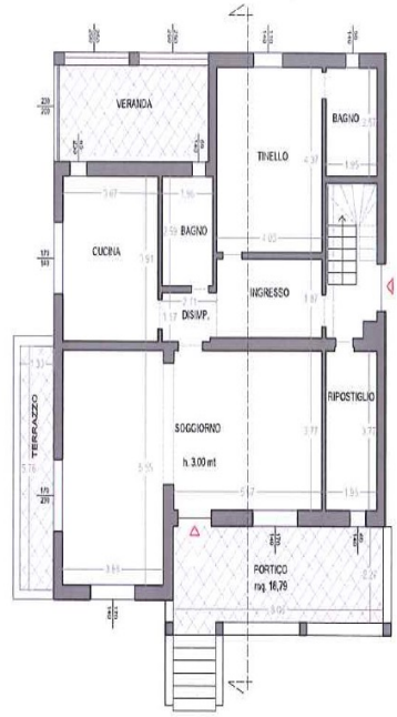
PIANO TERRA
