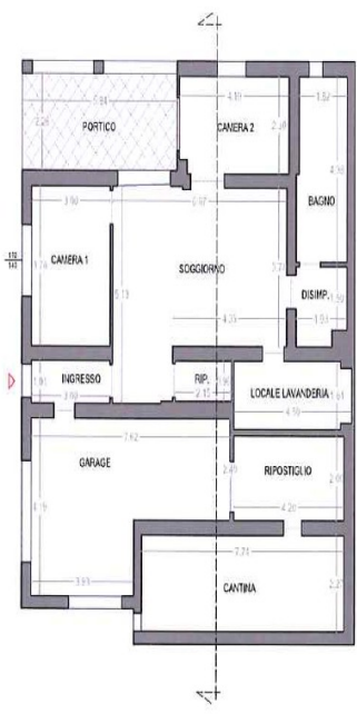
PIANO SEMINTERRATO
